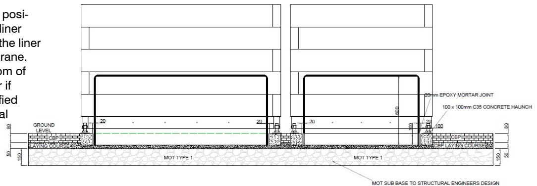
CT BLOCK (WITH GUNWHARF PLANTER) BLOCK PAVING INSTALLATION
