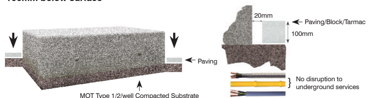
The CT Block sits only 100mm below surface
