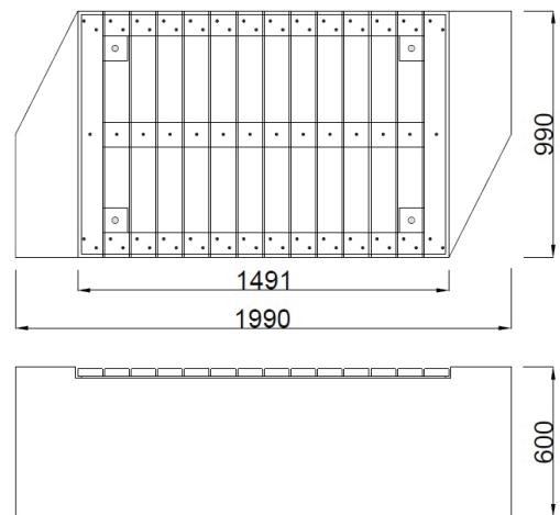
The CT Block sits only 100mm below surface
