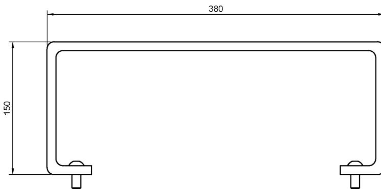
Stainless Steel Armrest for Blocks without a Backrest
